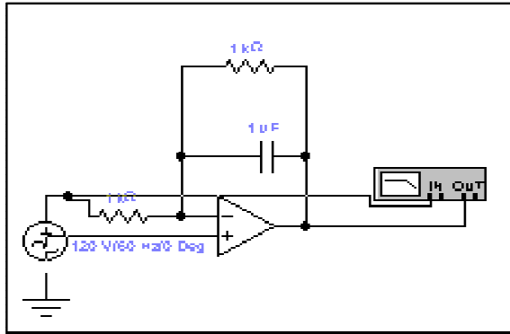
Gambar 2.16 Rangkaian Low Pass Filter aktif
