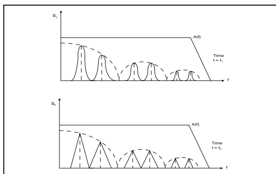
Gambar 2.3 : Konfigurasi kanal pada TDM A(f) : Frequency response of the transmission channel
