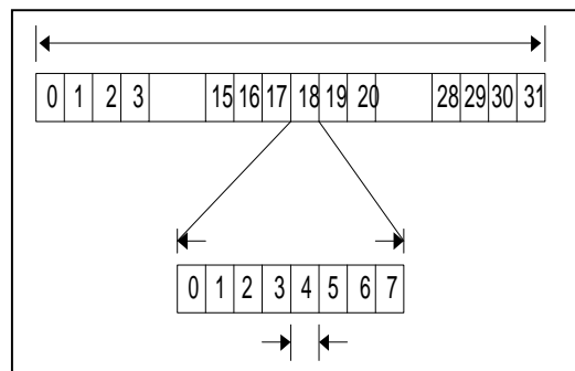
Gambar 2.4 : Pulse frame of the PCM 30/32
